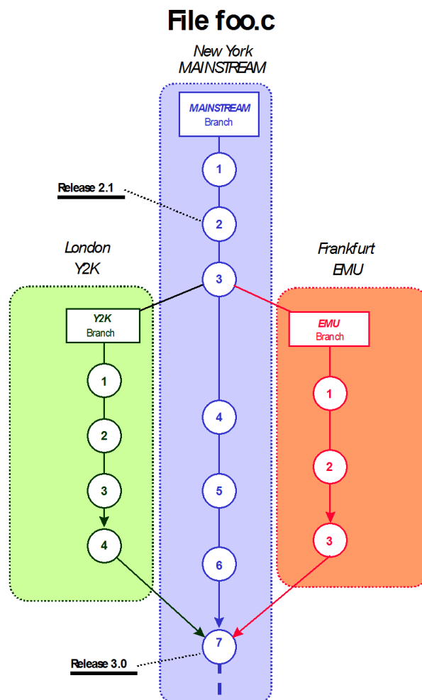
Figure 23-2. Multiple Named Branches
