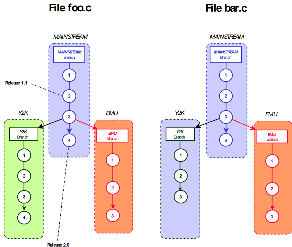
Figure 23-1. Version Trees, Releases and Branches
