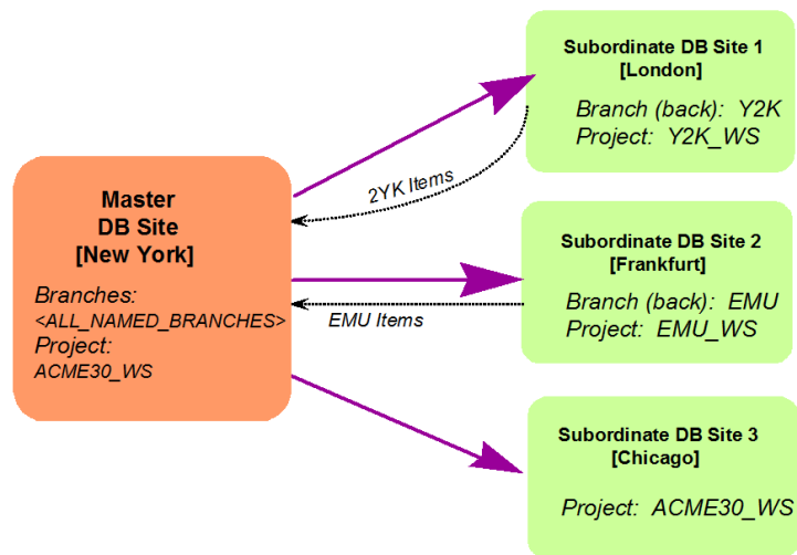
Figure 23-3. An Example Replication Configuration for a Master DB Site at New York
