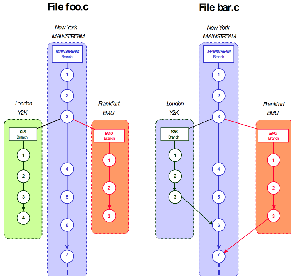
Figure 23-4. Example Item Pedigrees of Remotely Replicated Files
